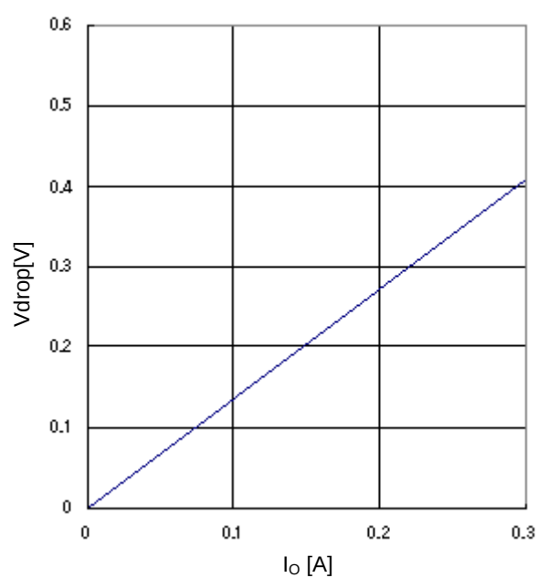
Figure 22. Minimum dropout Voltage 2 (Vcc=4.5V、Ta=25°C)
