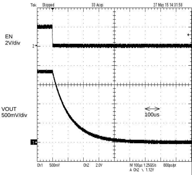
Figure 6. Shut down
