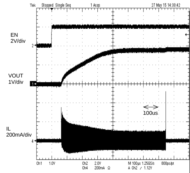
Figure 5. Start up
