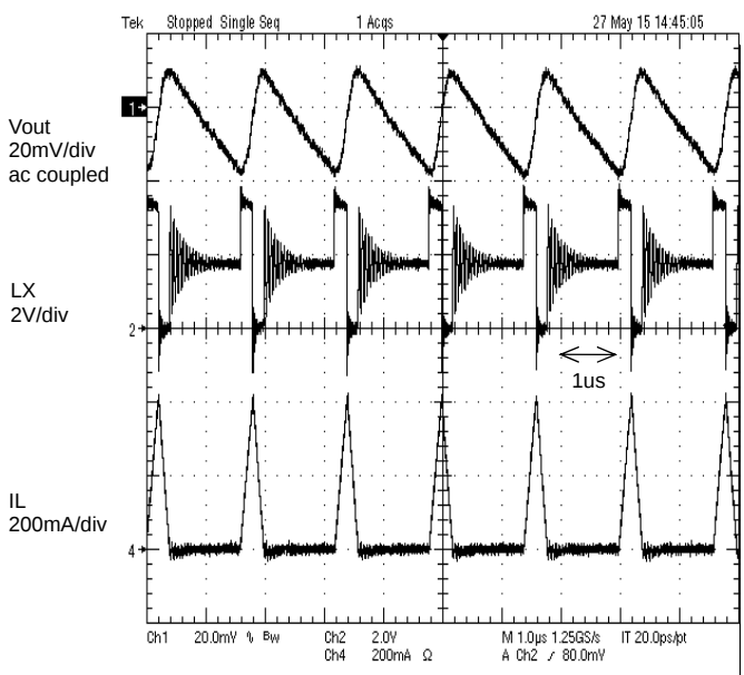
Figure 10. PFM mode Operation I_{out}=50\text{mA}
