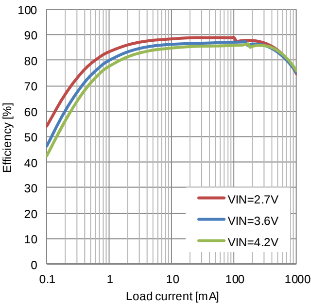
Figure 14. Efficiency vs Load current PWM/PFM Auto mode
