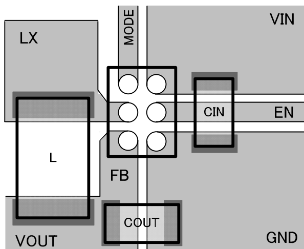
Figure 16. PCB layout
