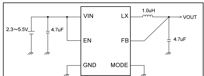
Figure 1. Typical Application Circuit(s)
