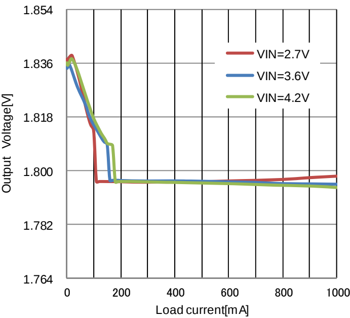
Figure 15. Load regulation PWM/PFM Auto mode
