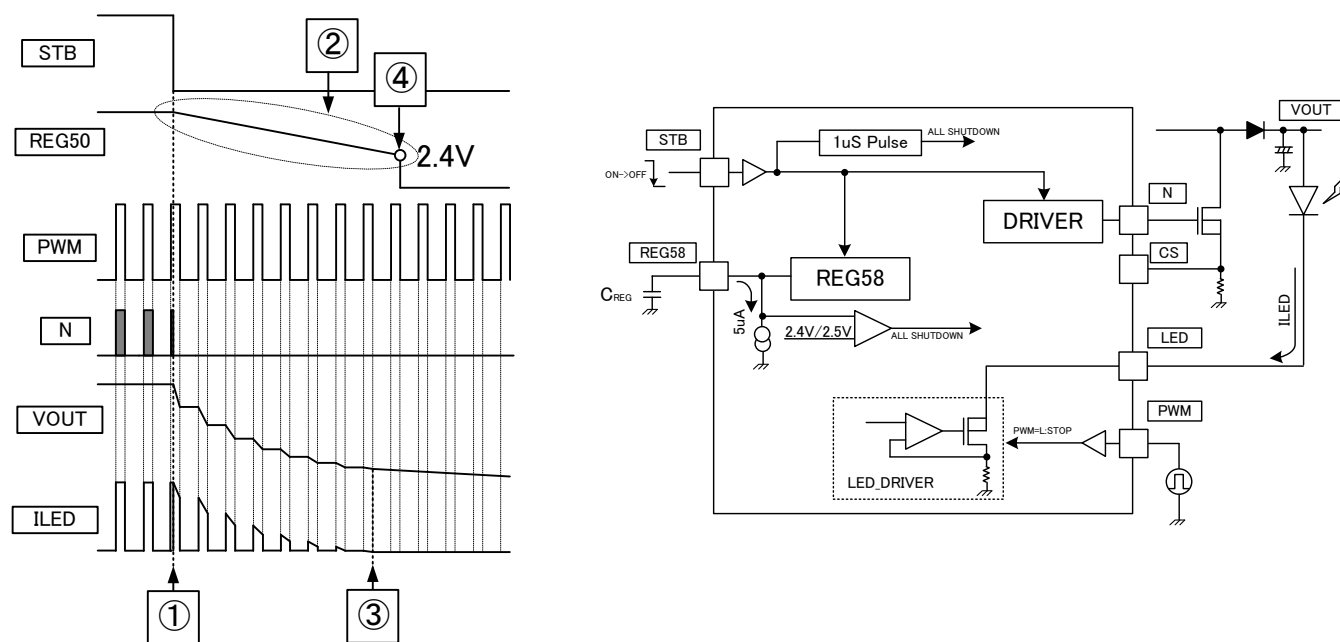
Figure 18. Timing chart of shutdown
