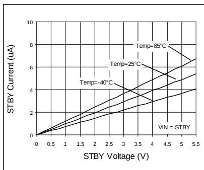
Fig. 99 STBY Input Current
