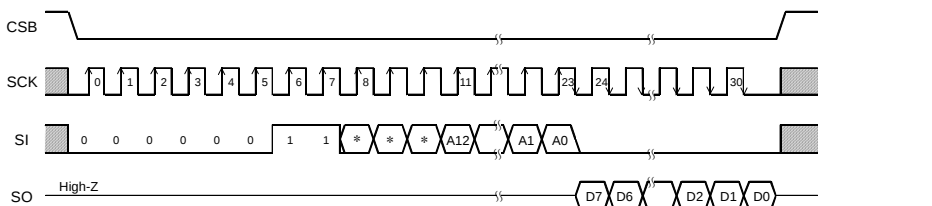
Figure 37. Read command
