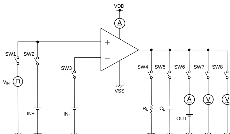
Figure 24. Test Circuit 2
