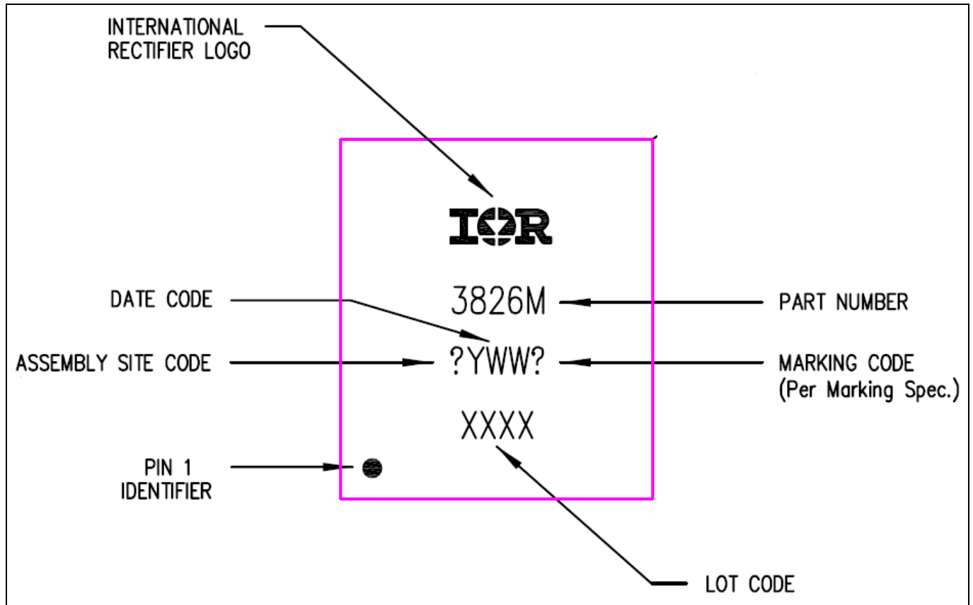
Figure 36 Package Marking
