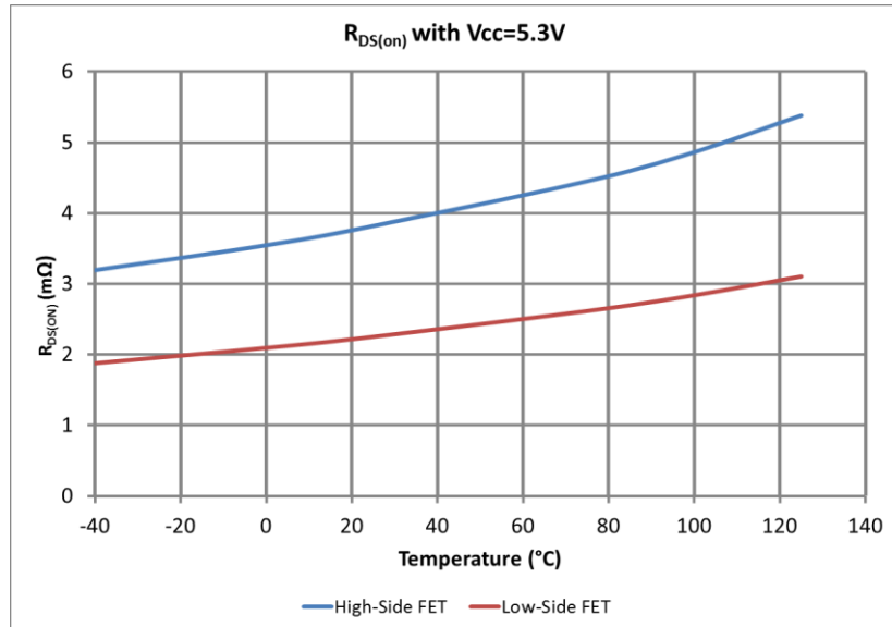
Figure 5 R DS(on) of MOSFETs over Temperature
