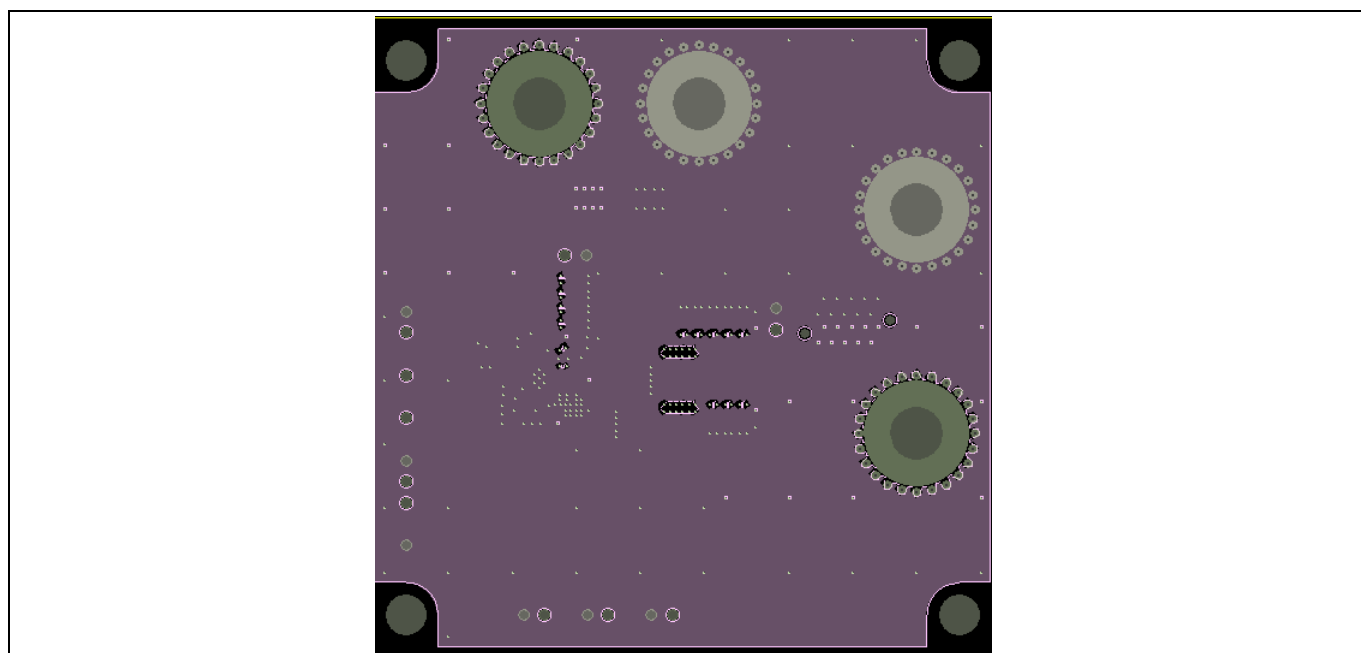
Figure 33 IRDC3826 Demo Board – Middle Layer 4 (Ground)
