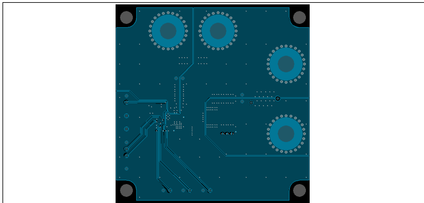
Figure 32 IRDC3826 Demo Board – Middle Layer 3 (Ground & Signal)
