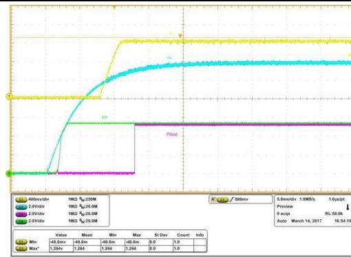
Start up at 23 A Load Ch1:V out , Ch2:PV in , Ch3:P Good , Ch4: V cc
