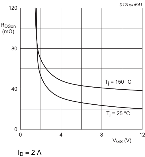
Fig 8. TR1: Drain-source on-state resistance as a function of gate-source voltage; typical values
