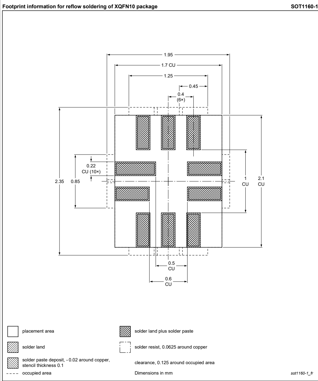
Figure 19. SOT1160-1 (XQFN10) footprint information for reflow soldering
