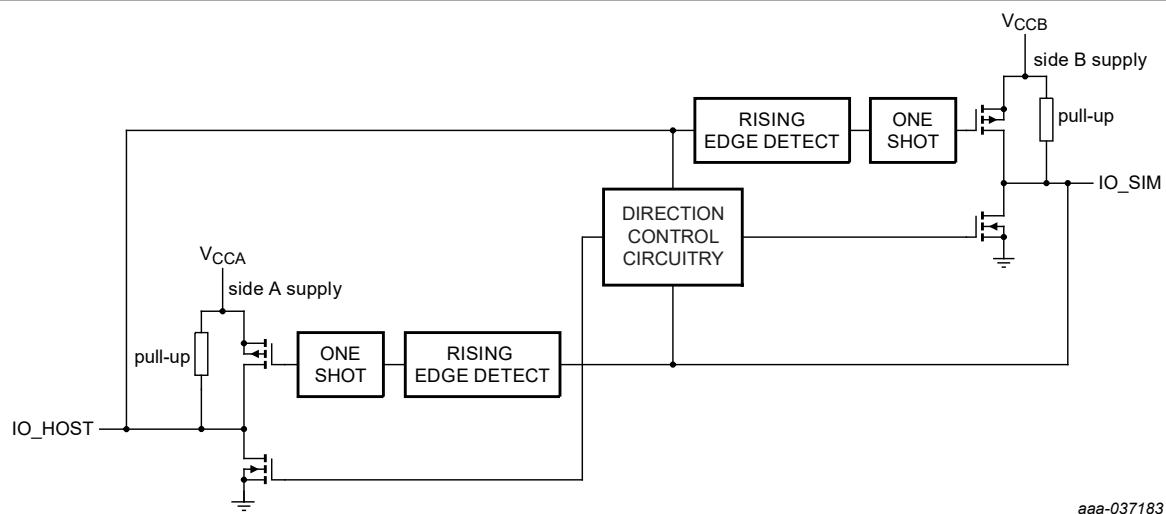
Figure 12. Automatic direction control level translator for HIGH-level direction change interfaces
