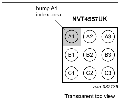
Figure 2. Bump configuration for WLCSP9
