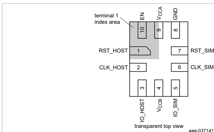
Figure 4. Pin configuration for XQFN10
