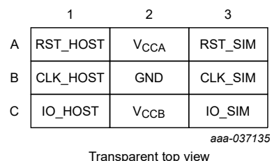
Figure 3. Bump mapping for WLCSP9
