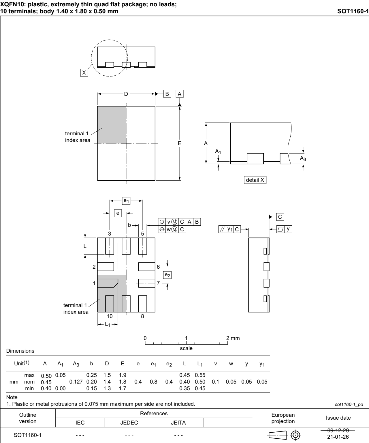
Figure 18. Package outline XQFN10 (SOT1160-1)
