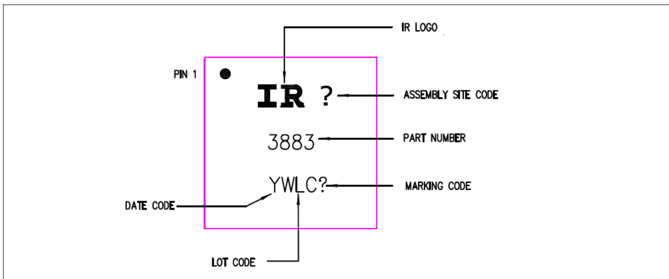
Figure 8-7 Marking information
