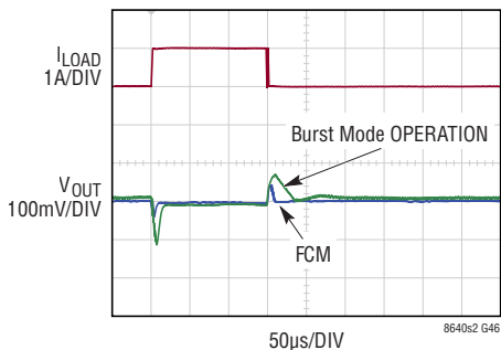
LT8643S-2 Transient Response; 100mA to 1.1A Transient
