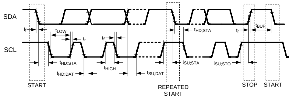
Figure 2. I²C Serial Control Bus Timing
