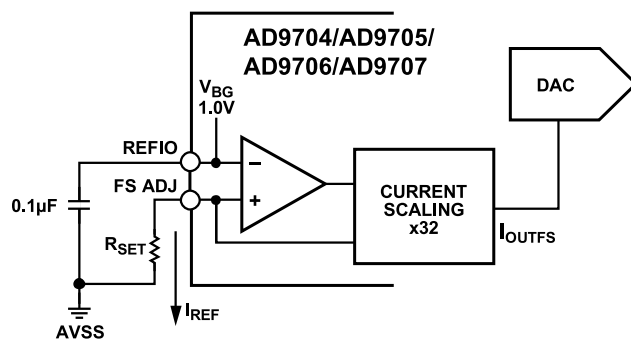
Figure 77. Internal Reference Configuration
