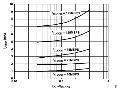
Figure 82. I_{DVDD} vs. f_{OUT}/f_{CLOCK} Ratio at DVDD = 3.3 V
