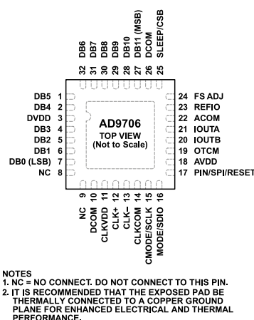
Figure 4. AD9706 Pin Configuration
