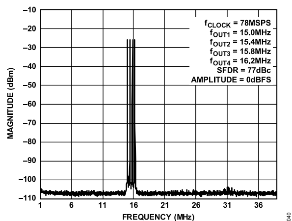
Figure 26. Four-Tone SFDR
