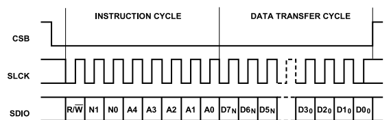
Figure 71. Serial Register Interface Timing, MSB First Write
