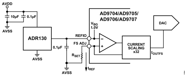
Figure 78. External Reference Configuration
