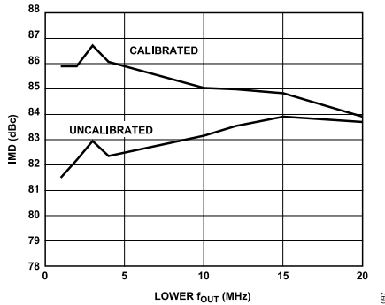
Figure 87. IMD vs. Lower f_{OUT} at 175 MSPS and I_{OUTS} = 2 mA
