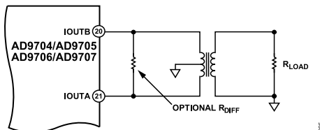
Figure 88. Differential Output Using a Transformer
