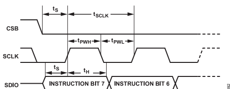
Figure 75. Timing Diagram for SPI Register Write
