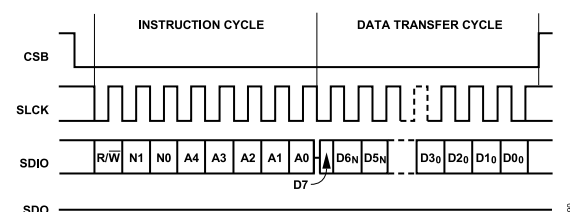
Figure 72. Serial Register Interface Timing, MSB First Read
