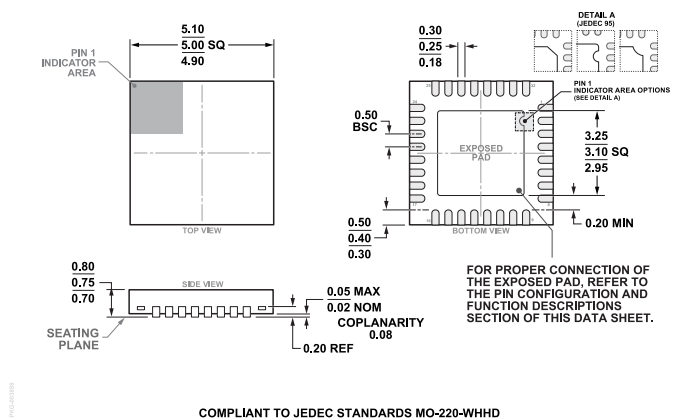
Figure 91. 32-Lead Lead Frame Chip Scale Package [LFCSP] 5 mm × 5 mm and 0.75 mm Package Height (CP-32-7) Dimensions shown in millimeters
