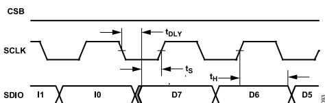
Figure 76. Timing Diagram for SPI Register Read
