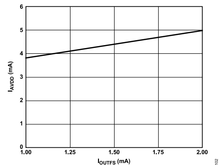
Figure 81. I_{AVDD} vs. I_{OUTFS} at AVDD = 1.8 V
