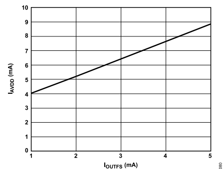
Figure 80. I_{AVDD} vs. I_{OUTFS} at AVDD = 3.3 V
