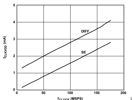
Figure 84. I_{CLKVDD} vs. f_{CLOCK} at CLKVDD = 3.3\text{ V}
