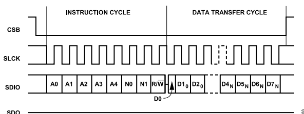
Figure 74. Serial Register Interface Timing, LSB First Read
