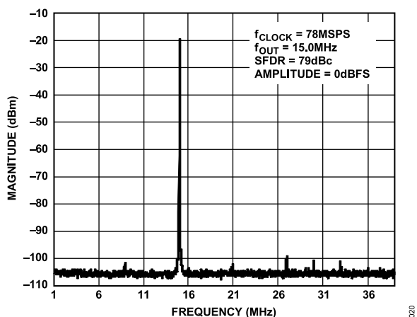
Figure 41. Single-Tone SFDR
