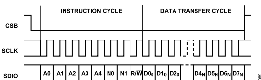
Figure 73. Serial Register Interface Timing, LSB First Write
