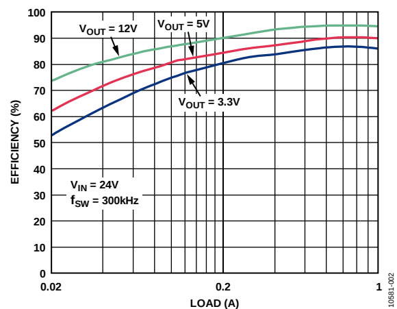
Figure 2. Efficiency vs. Load Current, V_{\text{IN}} = 24\text{V}
