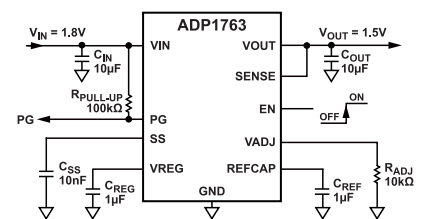
Figure 2. Adjustable Output Operation
