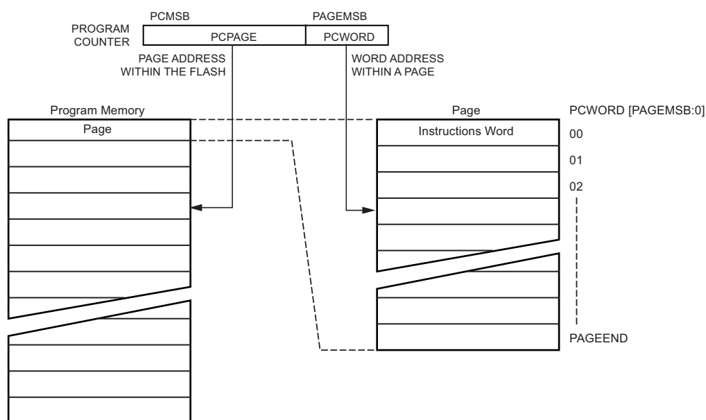
Figure 5-118. Addressing the Flash Which is Organized in Pages (1)
