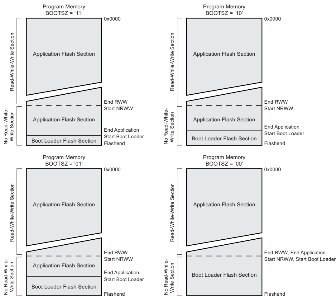
Figure 5-115. Memory Sections
