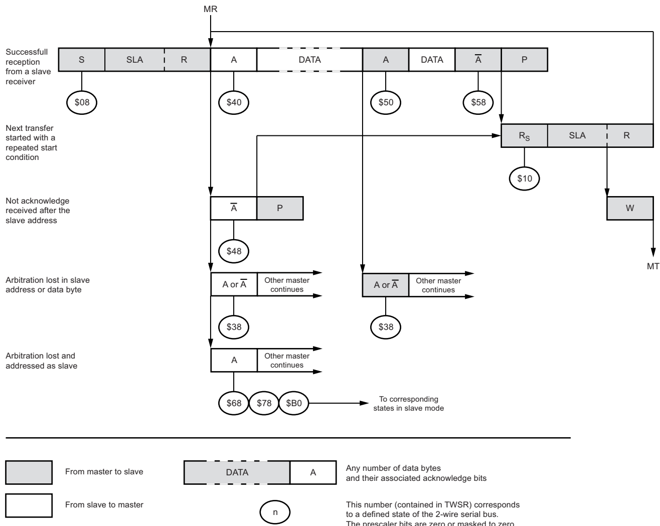
Figure 5-91. Formats and States in the Master Receiver Mode
