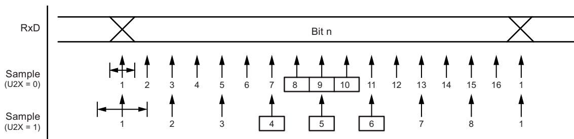
Figure 5-74. Sampling of Data and Parity Bit
