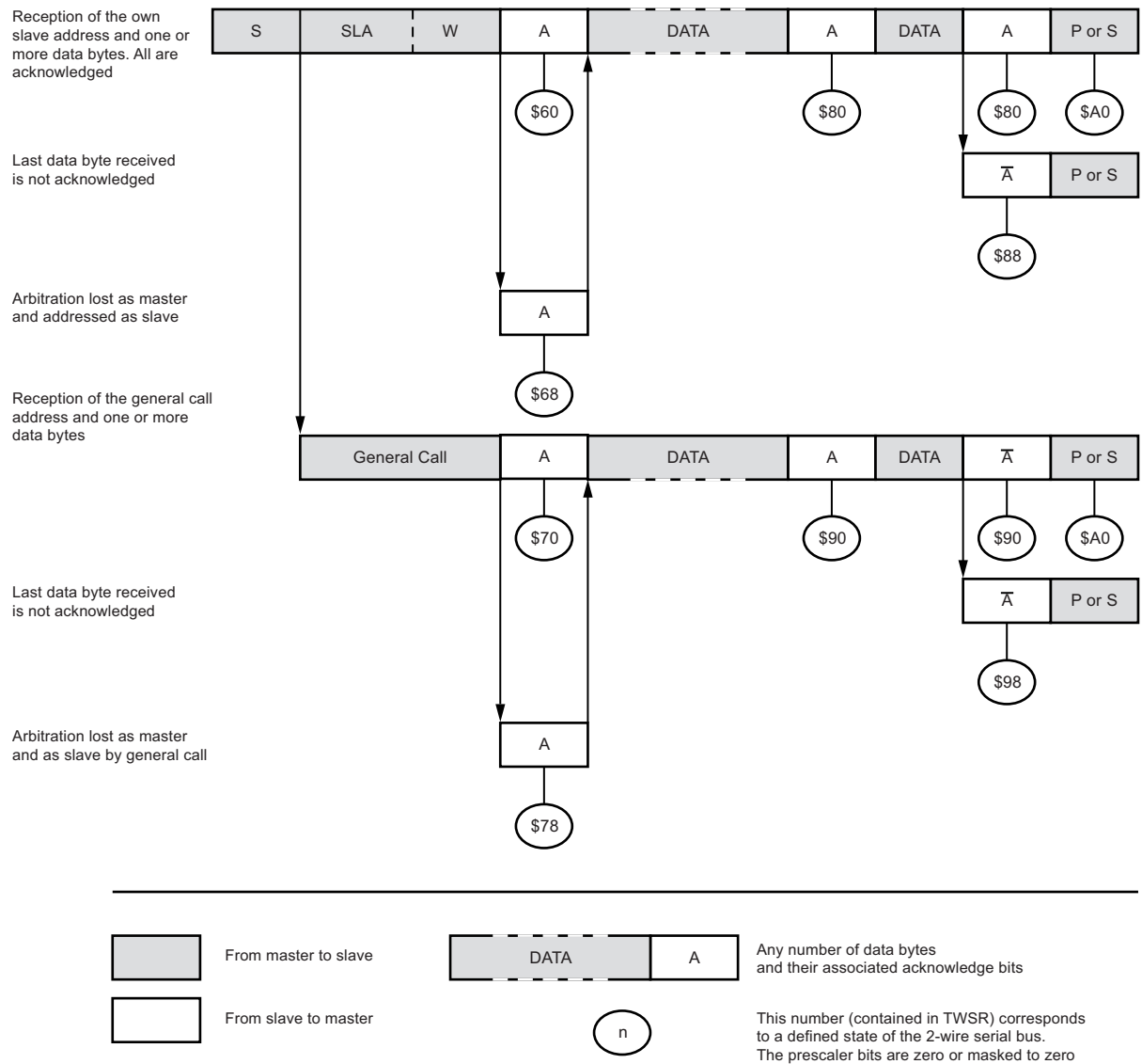
Figure 5-93. Formats and States in the Slave Receiver Mode
