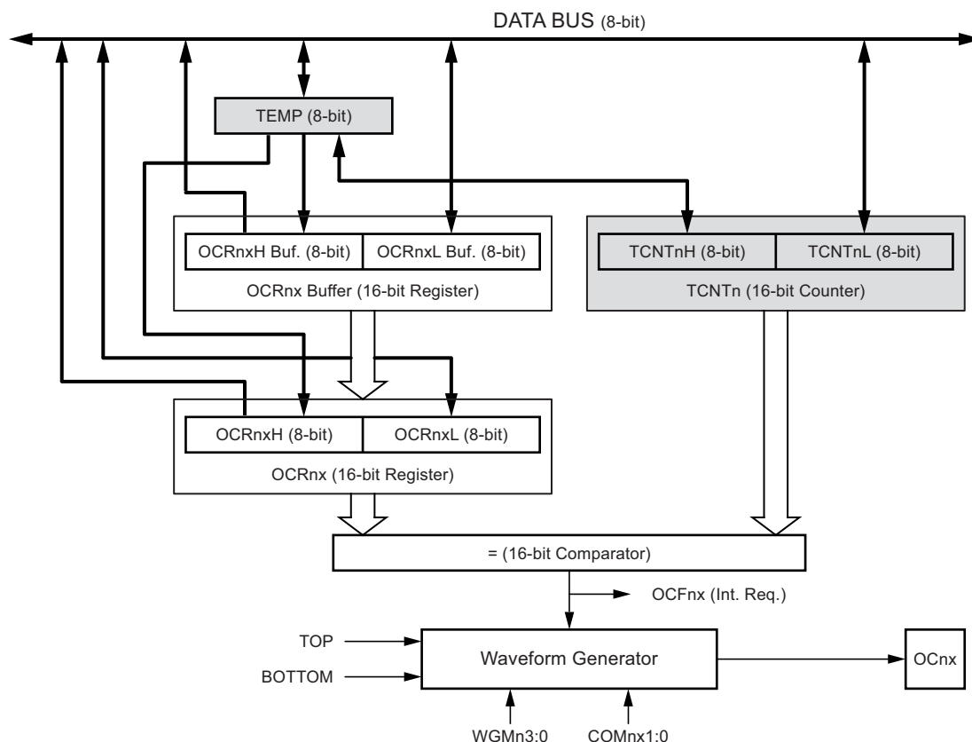
Figure 5-43. Output Compare Unit, Block Diagram
