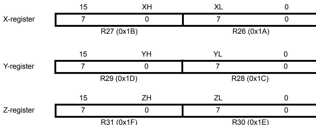
Figure 5-4. The X-, Y-, and Z-registers
