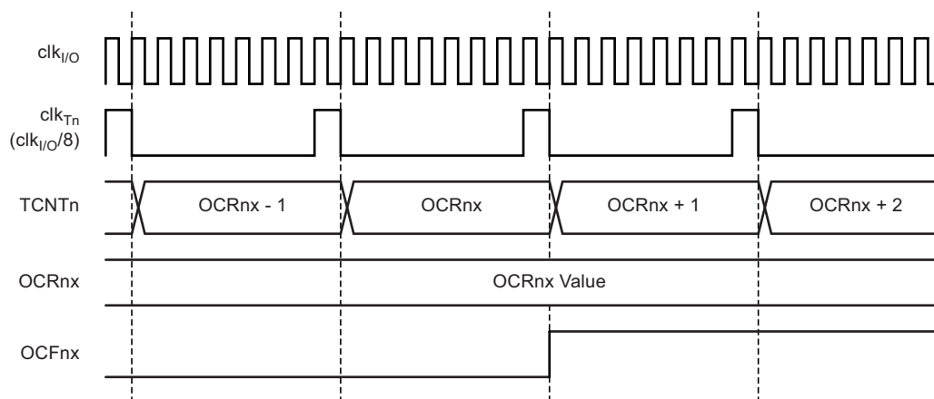
Figure 5-50. Timer/Counter Timing Diagram, Setting of OCF1x, with Prescaler ( f_{\text{clk\_I/O}}/8 )
