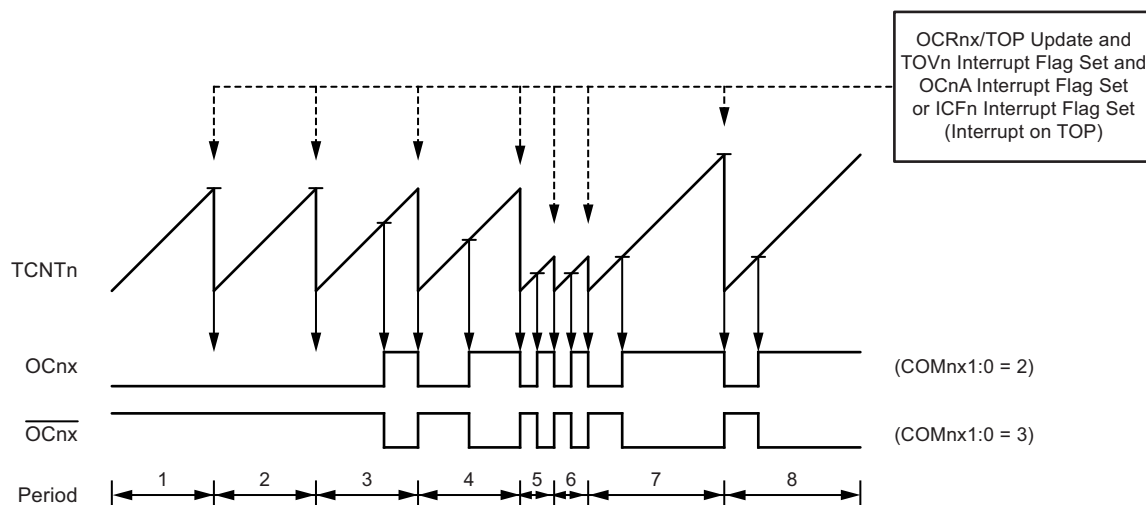
Figure 5-46. Fast PWM Mode, Timing Diagram
