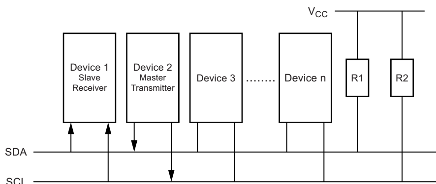
Figure 5-92. Data Transfer in Slave Receiver Mode
