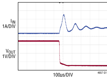
Short-Circuit with No Load Applied
