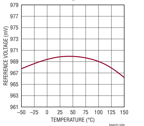
Reference Voltage
