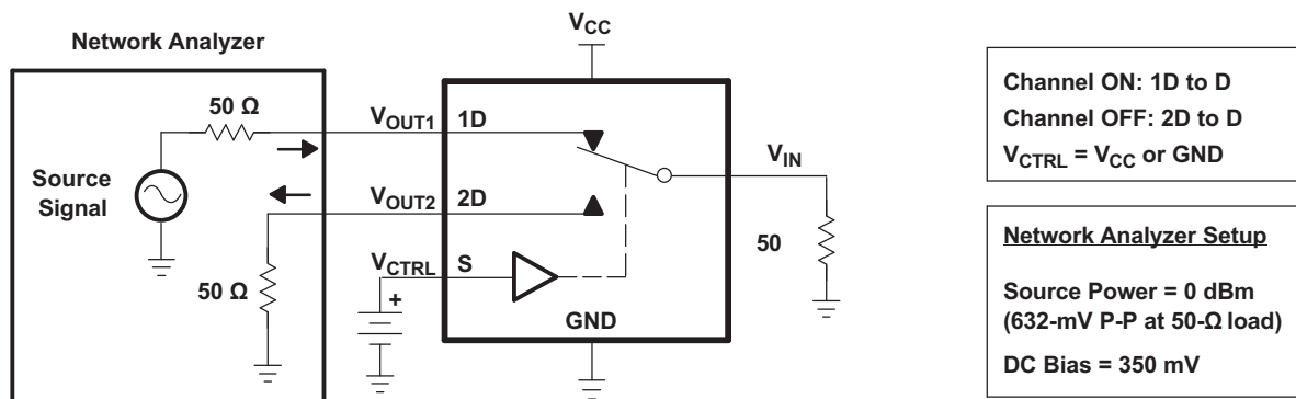
Figure 8. Crosstalk ( X_{TALK} )
