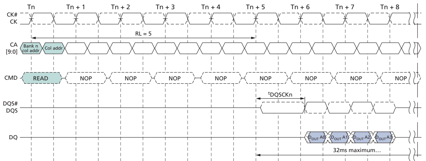
Figure 17: t_{DQSKDL} Timing
