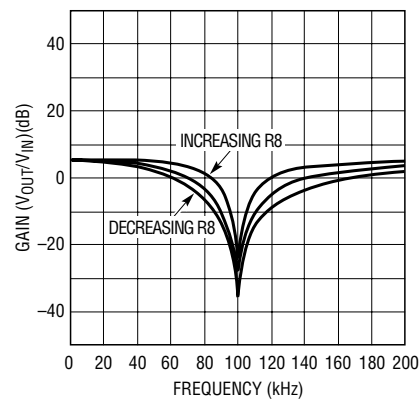
Figure 6. Frequency Response
