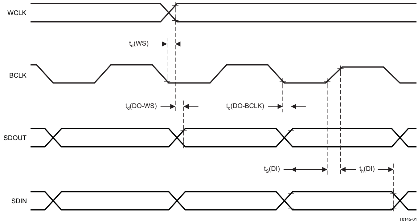
Figure 1. I²S, Left-Justified and Right-Justified Format Timing in Master Mode
