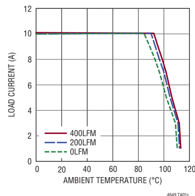
Current Derating: 12V Input, 1.5VOUT, No Heat Sink
