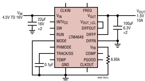
4.5V to 16V Input, 1.5V Output DC/DC \mu Module Regulator
