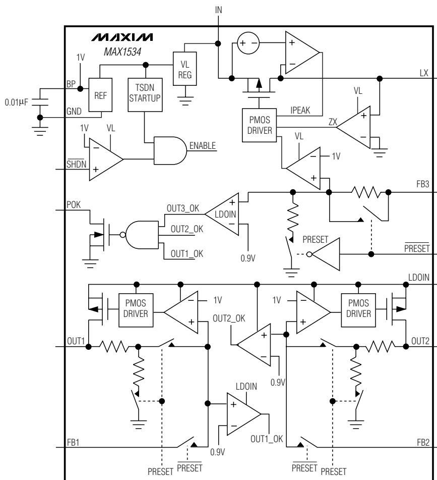
Figure 2. MAX1534 Functional Block Diagram
