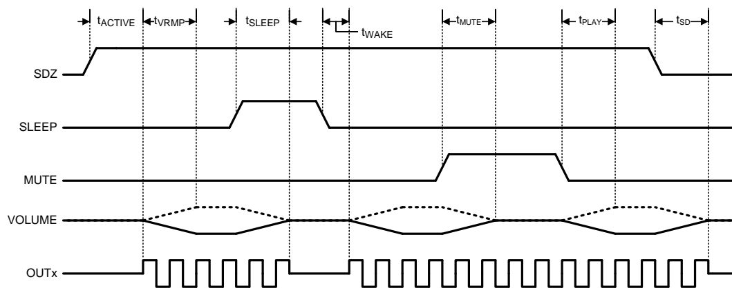
Figure 4. Mode Timing
