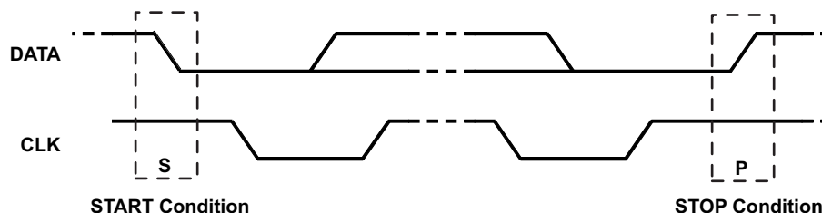
Figure 21. START and STOP Condition
