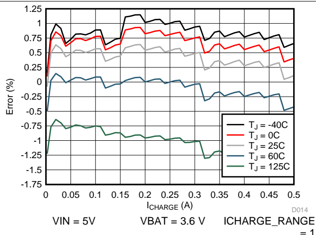
Figure 2. Charge Current Accuracy vs. ICHARGE setting
