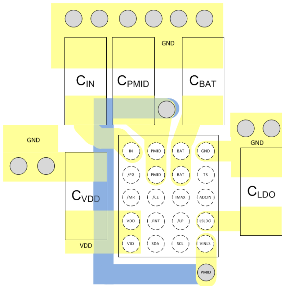
Figure 101. Layout Example
