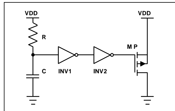
Figure 17. 5173 Supply Clamp Structure
