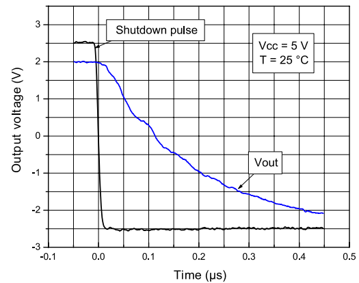
Figure 18: Turn-off time, V_{\text{CC}} = 5 V, Vout pulled down, T = 25 °C
