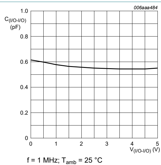
Fig. 3. Input/output to input/output capacitance as a function of input/output to input/output voltage; typical values
