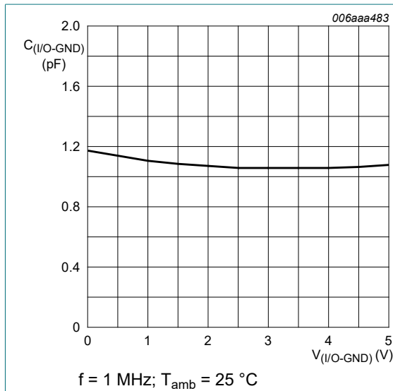
Fig. 2. Input/output to ground capacitance as a function of input/output to ground voltage; typical values
