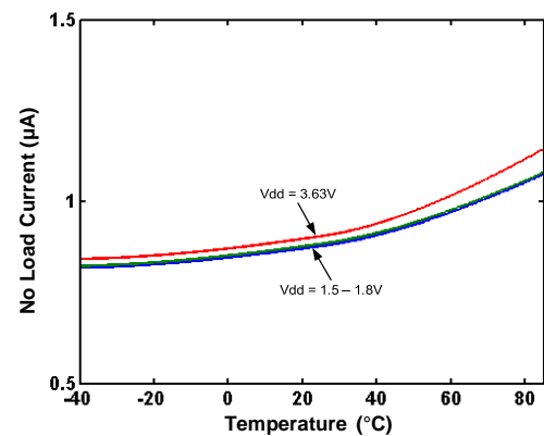
Figure 7. Supply Current Over Temperature (No Load)
