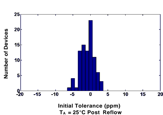
Figure 5. Initial Tolerance Histogram
