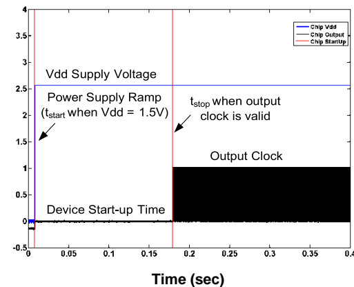
Figure 8. Start-up Time
