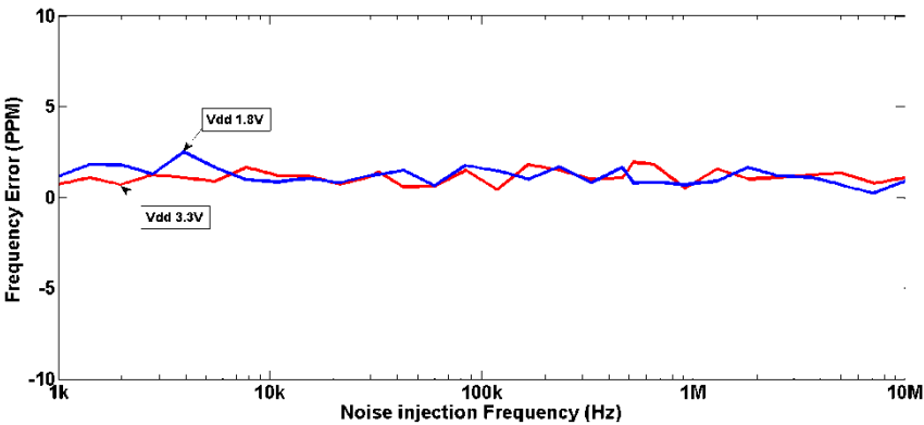
Figure 9. Power Supply Noise Rejection ( \pm 150\text{mV} Noise)
