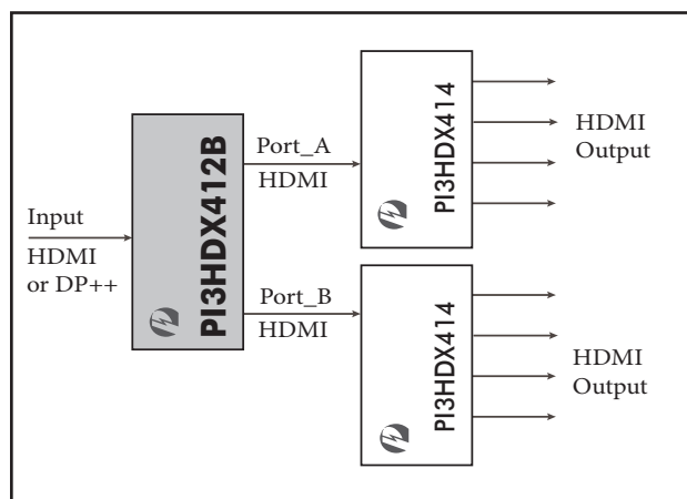
Application Block Diagram
