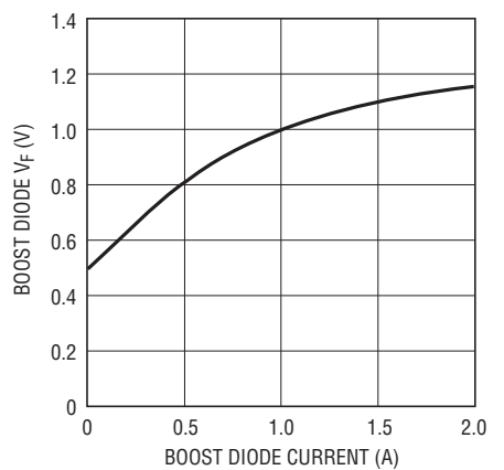
Boost Diode
