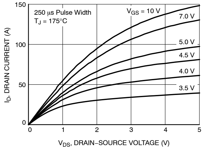
Figure 10. Saturation Characteristics
