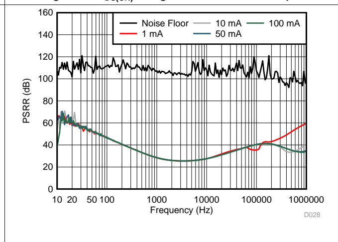
Figure 14. LS/LDO PSRR vs Frequency
