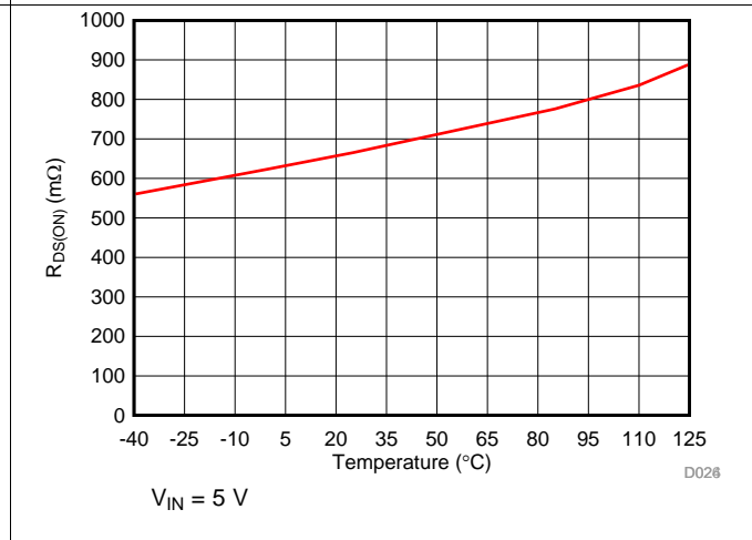
Figure 12. R_{DS(ON)} of High Side MOSFET vs Temperature
