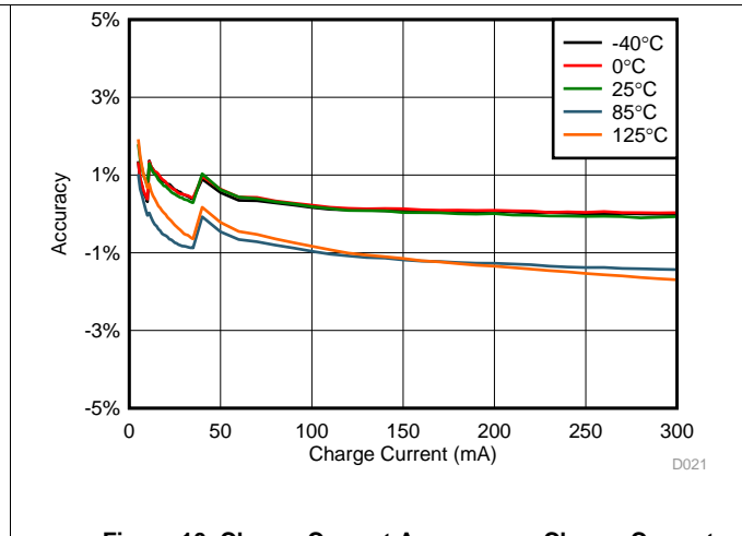
Figure 10. Charge Current Accuracy vs Charge Current
