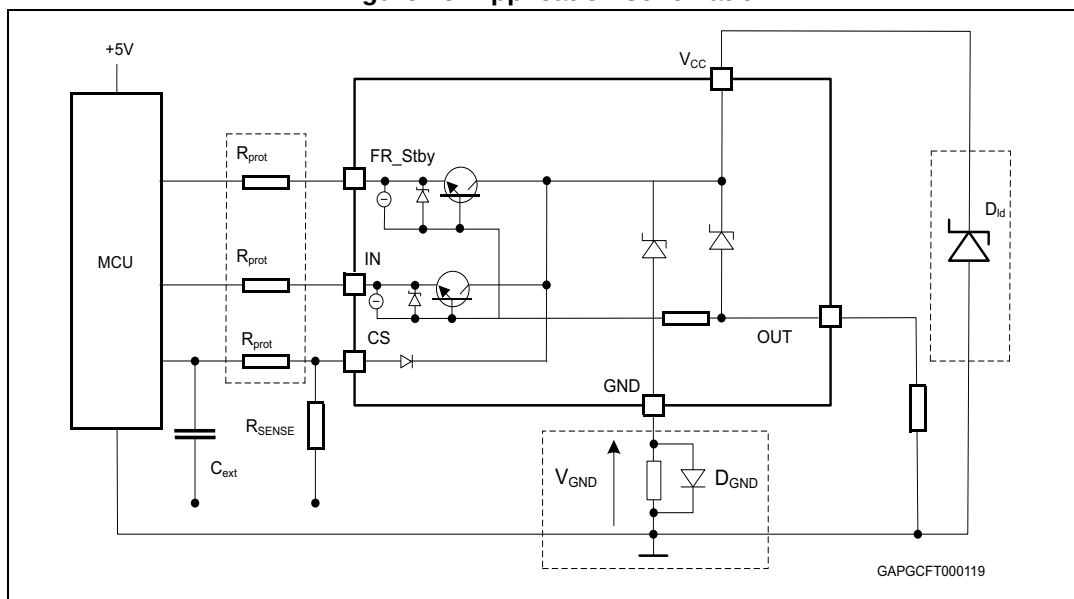
Figure 25. Application schematic
