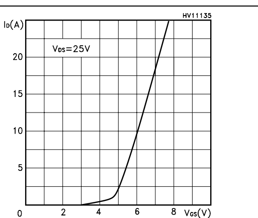
Figure 7. Transfer characteristics
