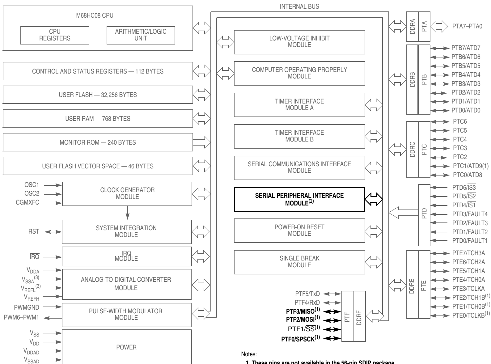
Figure 15-1. Block Diagram Highlighting SPI Block and Pins
