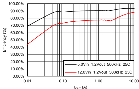
Figure 24. Efficiency Performance
