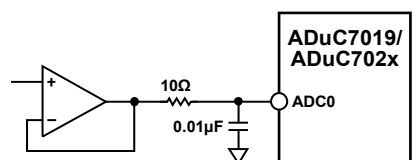
Figure 59. Buffering Single-Ended/Pseudo Differential Input
