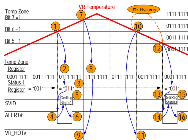
FIGURE 14. VR HOT#/ALERT# BEHAVIOR
