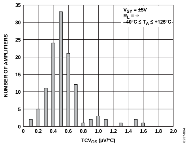
Figure 47. TCV_{OS} Distribution, LFCSP
