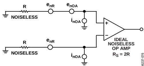
Figure 109. Op Amp Noise Circuit Model Used to Determine Total Circuit Equivalent Input Noise Voltage and Noise Figure
