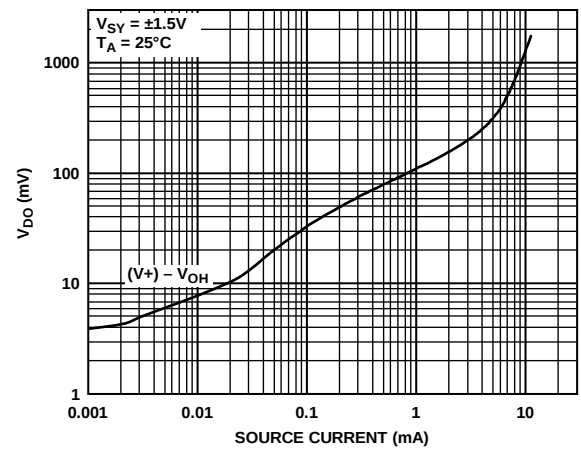
Figure 21. Dropout Voltage ( V_{DO} ) vs. Source Current
