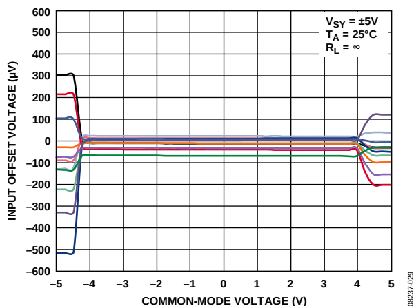
Figure 48. Input Offset Voltage vs. Common-Mode Voltage
