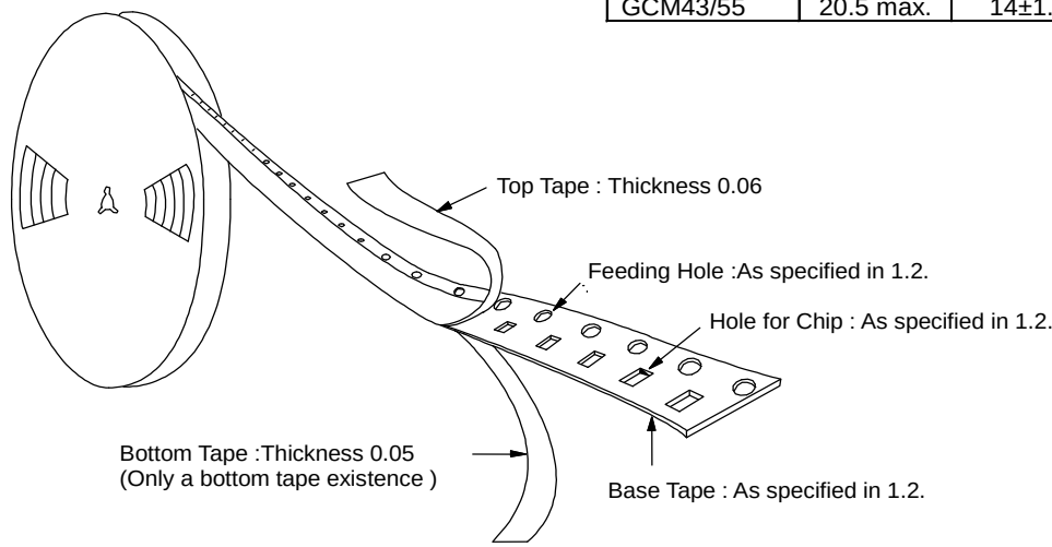
Fig.3 Taping Diagram
