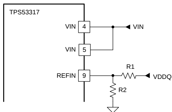
Figure 20. Tracking Configuration 2
