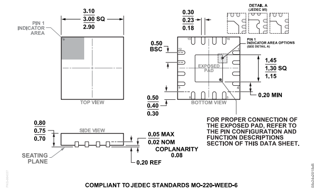
Figure 69. 16-Lead Lead Frame Chip Scale Package [LFCSP] 3 mm x 3 mm Body and 0.75 mm Package Height (CP-16-21) Dimensions shown in millimeters
