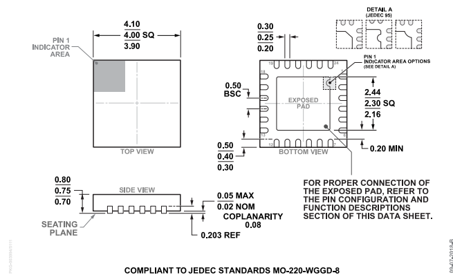
Figure 70. 24-Lead Lead Frame Chip Scale Package [LFCSP] 4 mm x 4 mm Body and 0.75 mm Package Height (CP-24-14) Dimensions shown in millimeters
