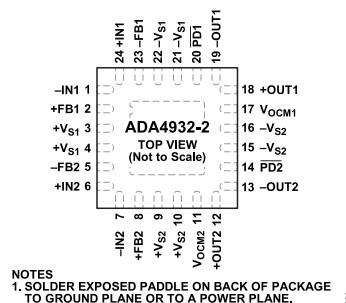
Figure 5. ADA4932-2 Pin Configuration
