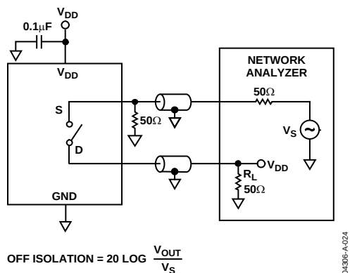
Figure 25. Off Isolation
