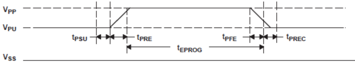
Figure 10. PROGRAM PULSE Timing Diagram
